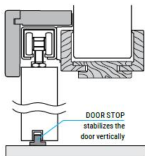
VERTICAL CROSS-SECTION OF THE SLIDING SYSTEM
